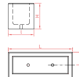
Bac rectangle Dim. : L80 x l40 x H40 cm - 162 kg L100 x l40 x H40 cm - 223 kg L120 x l40 x H50 cm - 348 kg L150 x l40 x H50 cm - 418 kg L150 x l40 x H45 cm - 400 kg L150 x l50 x H50 cm - 430 kg L150 x l60 x H60 cm - 585 kg L180 x l70 x H60 cm - 731 kg
